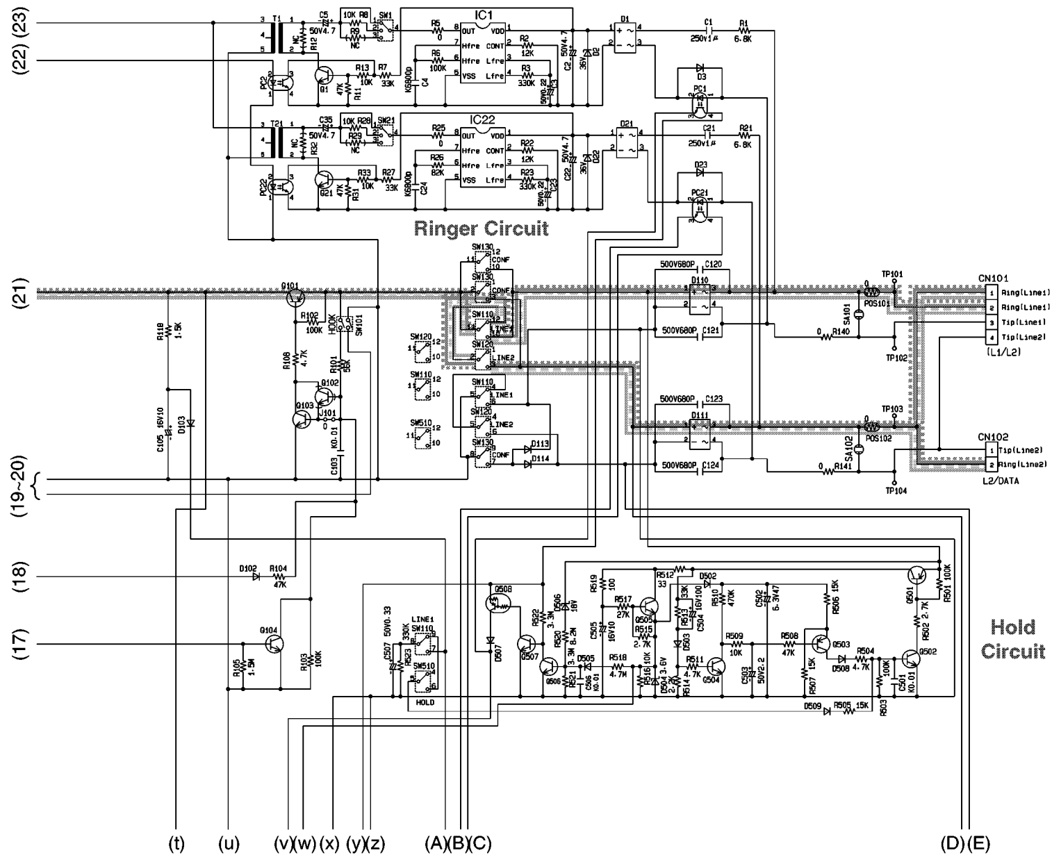
KX-T2378JXW SCHEMATIC DIAGRAM (Main (Suffix A)) 2/4
