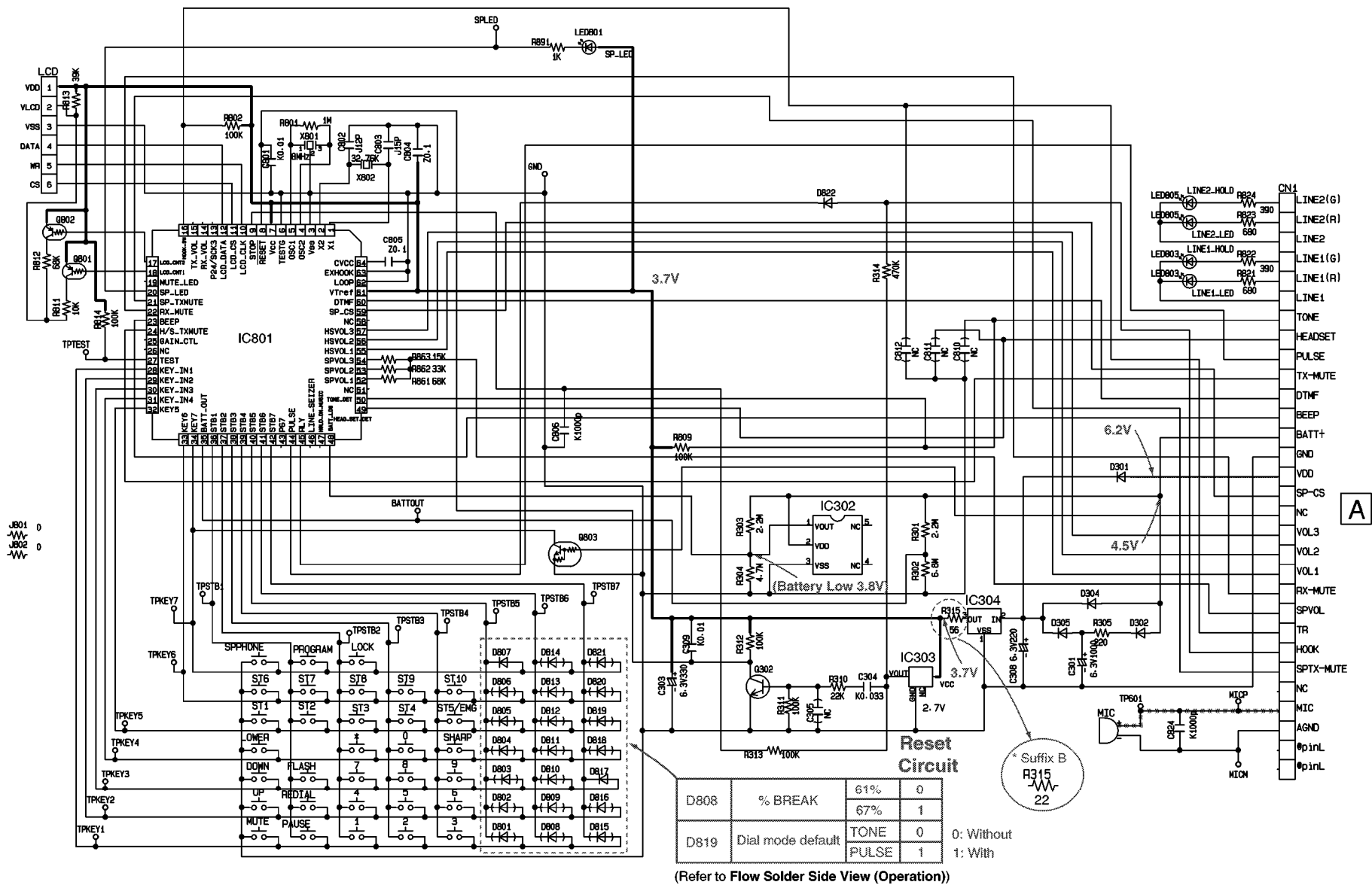
KX-T2378JXW SCHEMATIC DIAGRAM (Operation)
