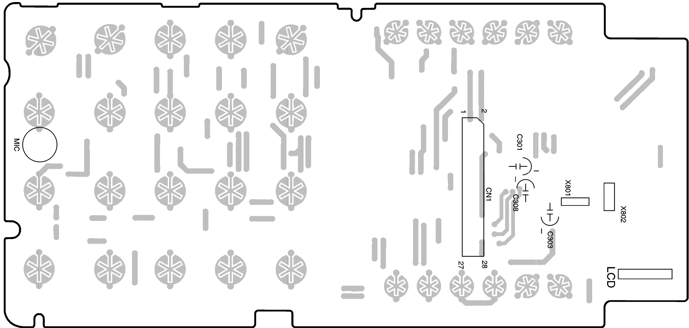
KX-T2378JXW CIRCUIT BOARD (Component View (Operation))
