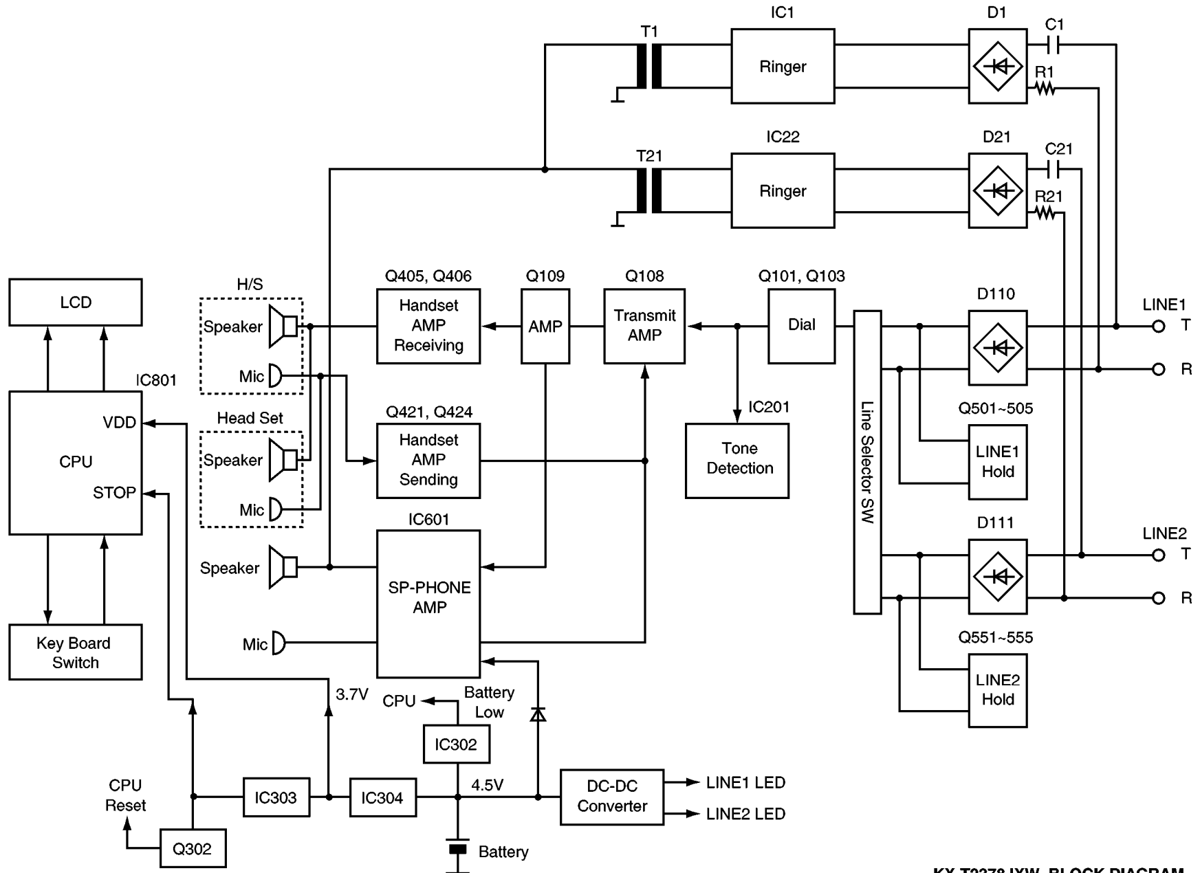
KX-T2378JXW BLOCK DIAGRAM
