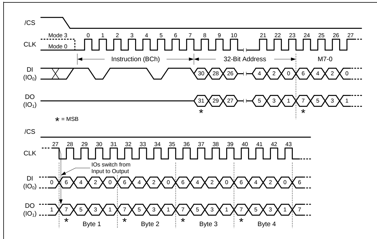
Figure 23a. Fast Read Dual I/O with 4-Byte Address Instruction (Initial instruction or previous M5-4 \neq 10, SPI Mode only)
