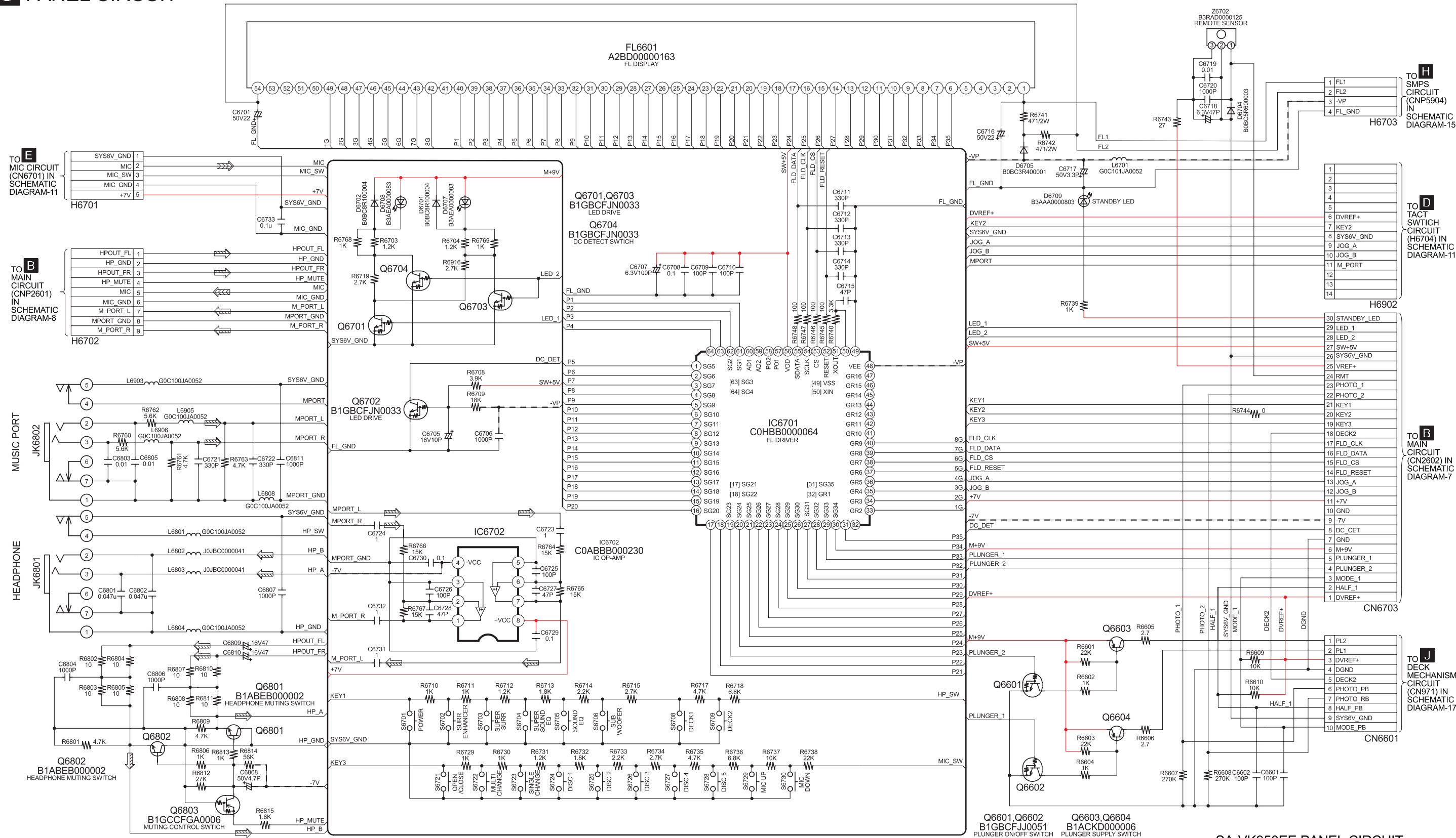
SA-VK950EE PANEL CIRCUIT
