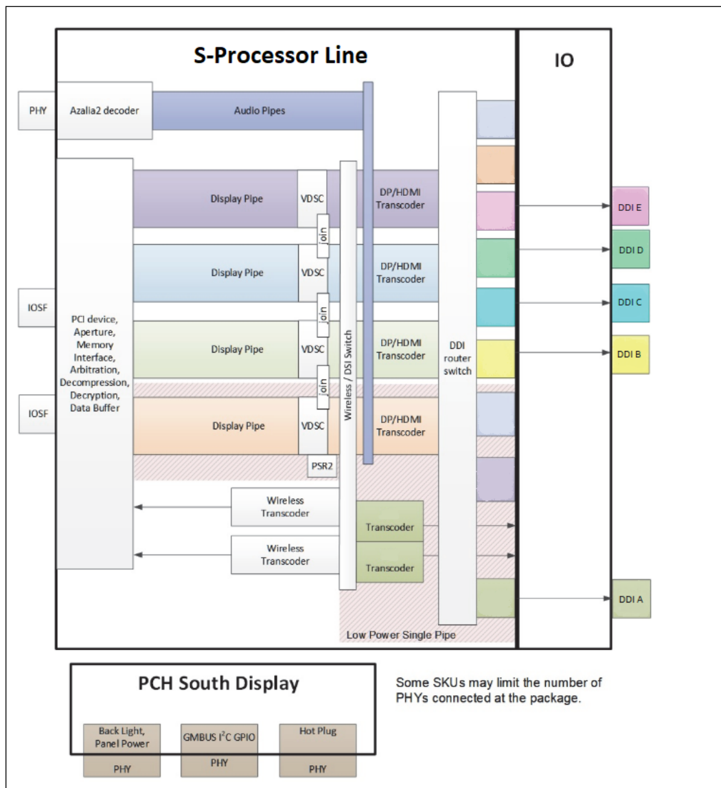
Figure 21. S/S Refresh, HX Processor Display Architecture
