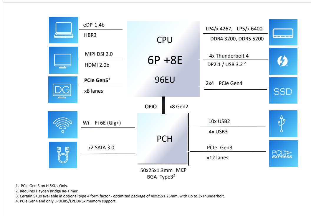
Figure 3. P/H Processor Line Platform Diagram
