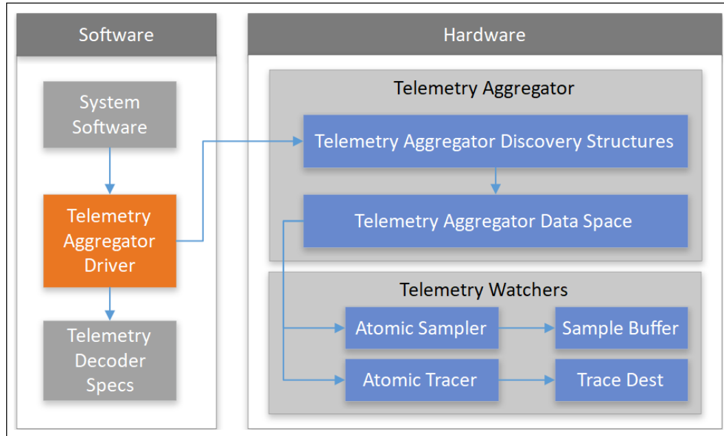
Figure 12. Telemetry Aggregator
