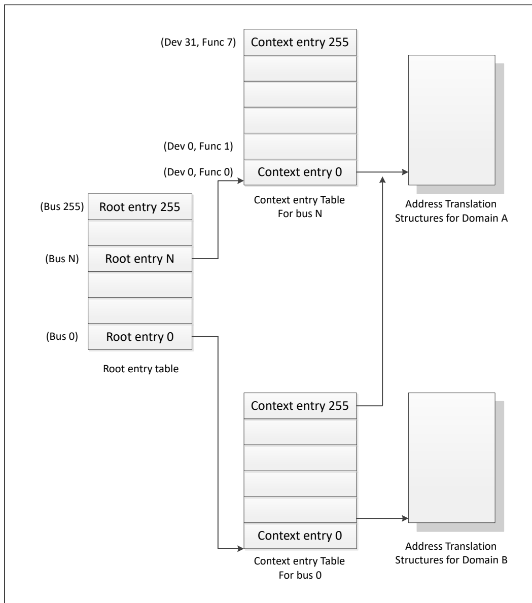
Figure 9. Device to Domain Mapping Structures
