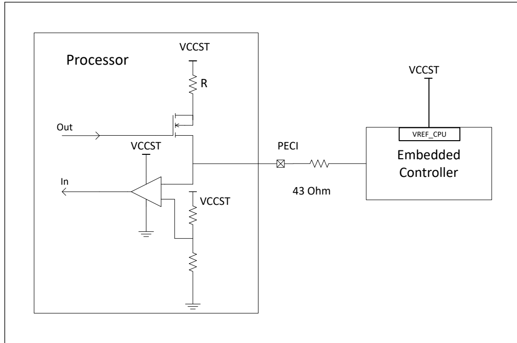
Figure 8. Example for PECI EC Connection
