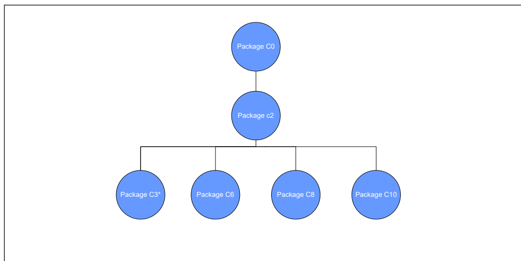
Figure 15. Package C-State Entry and Exit
