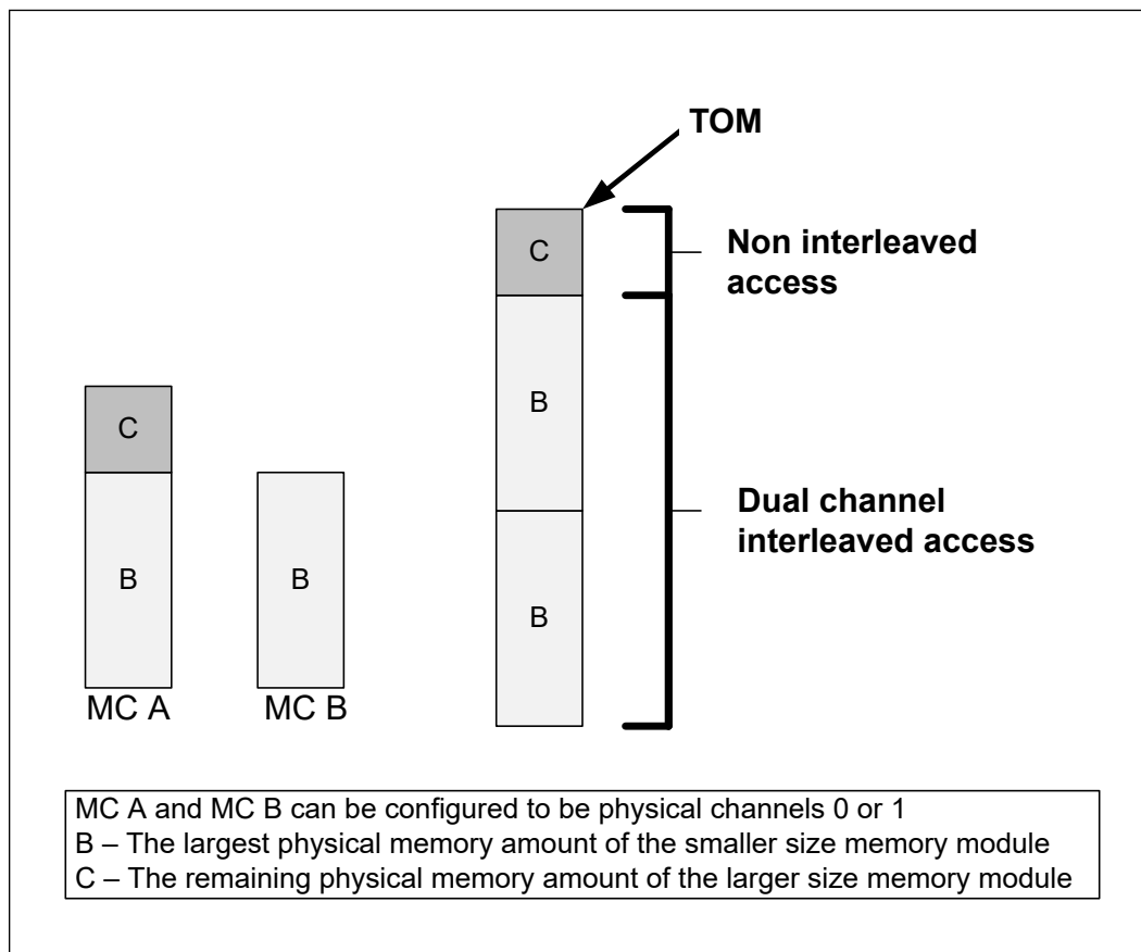
Figure 18. Intel® DDR4/5 Flex Memory Technology Operations
