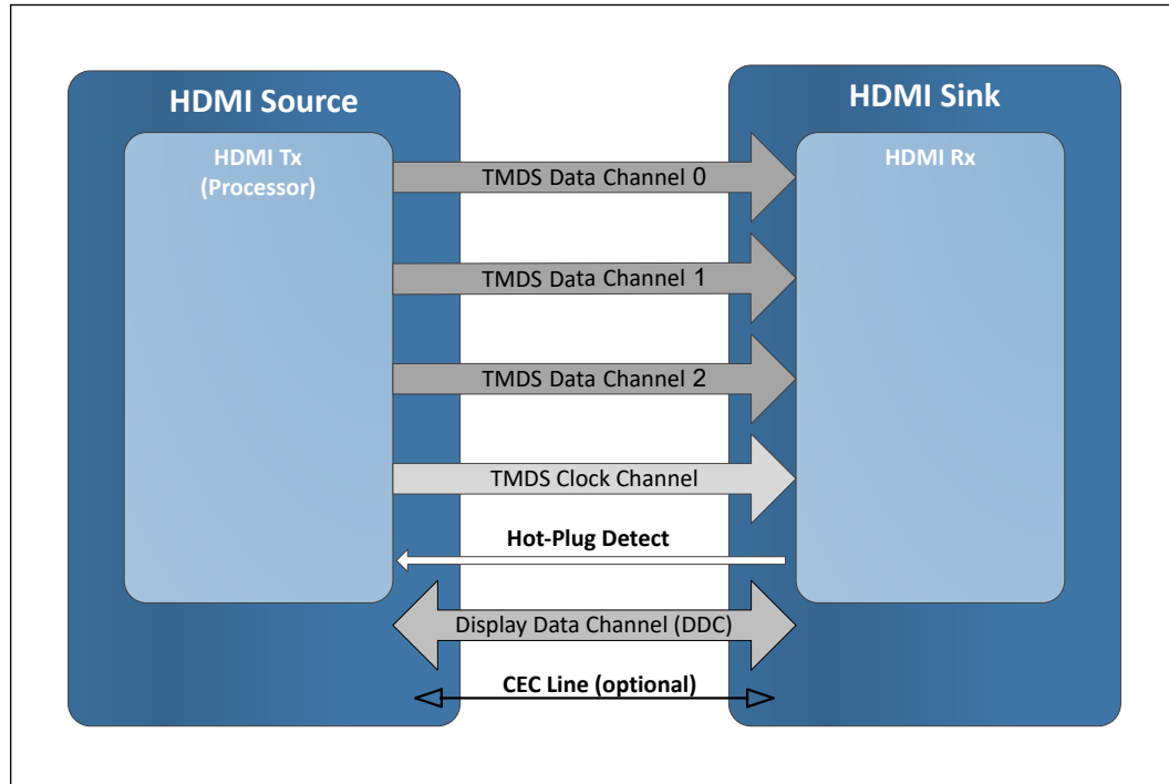
Figure 24. HDMI* Overview
