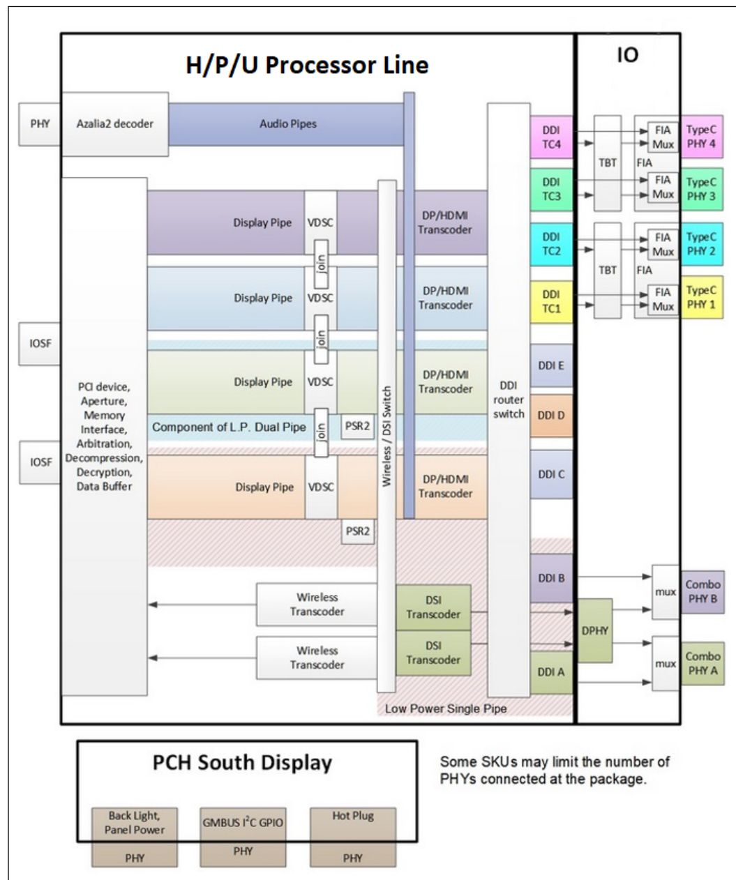
Figure 22. P, PX/U/H Processor Display Architecture
