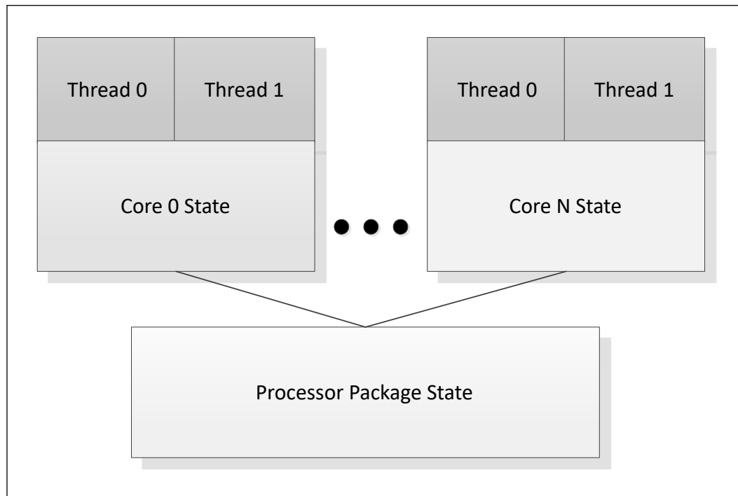
Figure 14. Idle Power Management Breakdown of the Processor IA Cores
