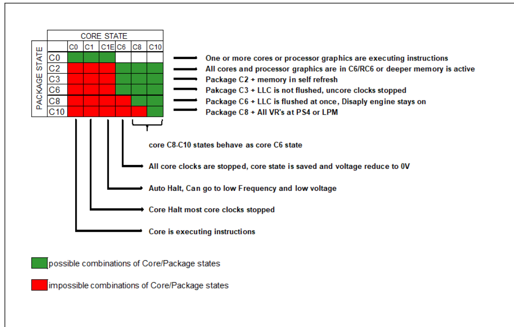
Figure 13. Processor Package and IA Core C-States
