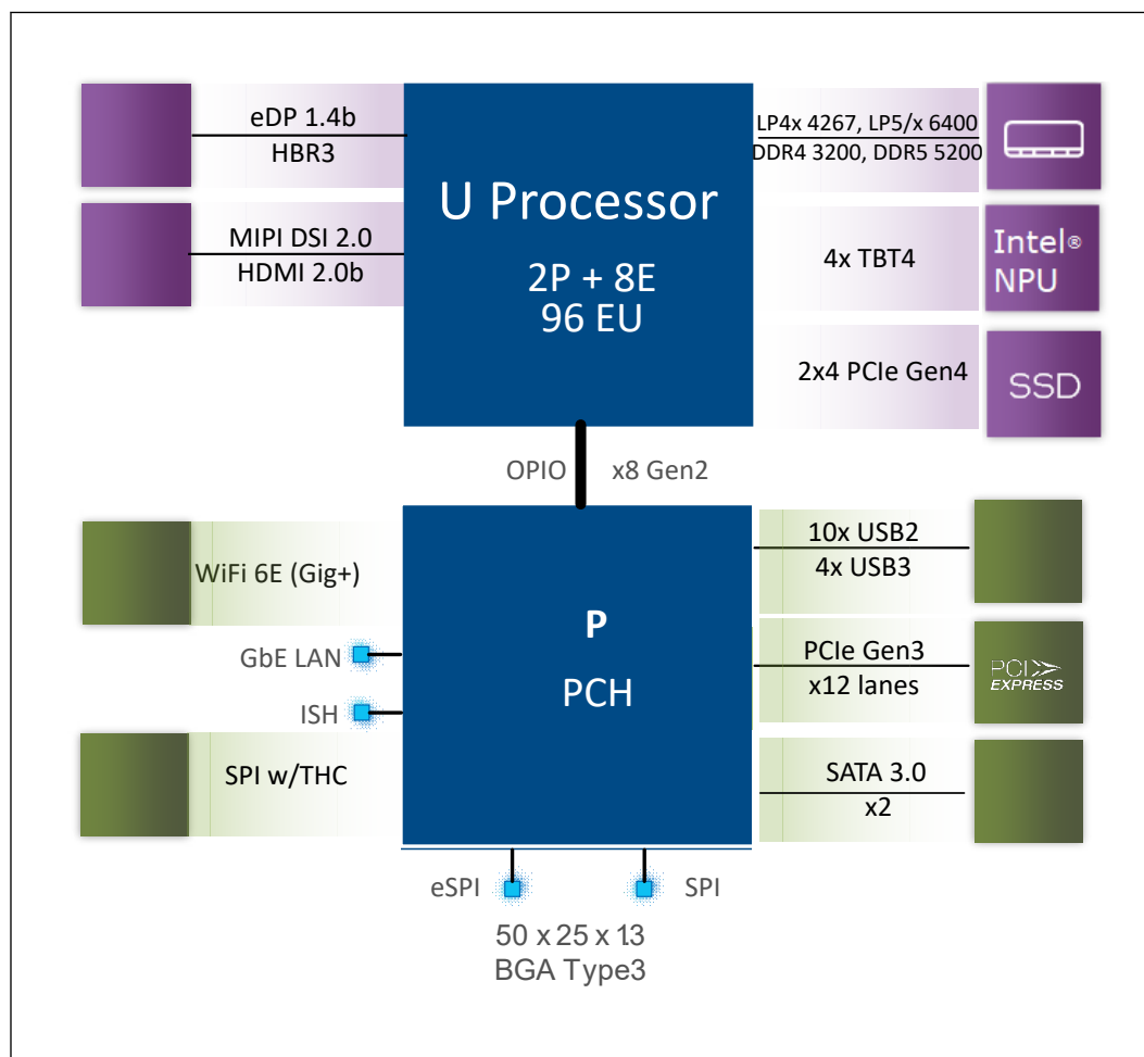
Figure 4. U Processor Line Platform Diagram
