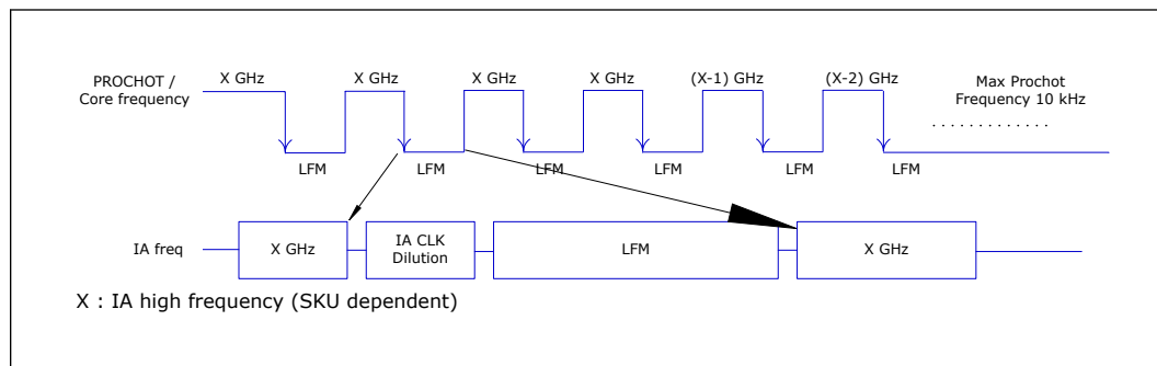
Figure 17. PROCHOT Demotion Description
