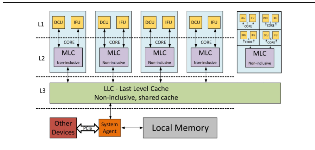
Figure 10. Hybrid Cache
