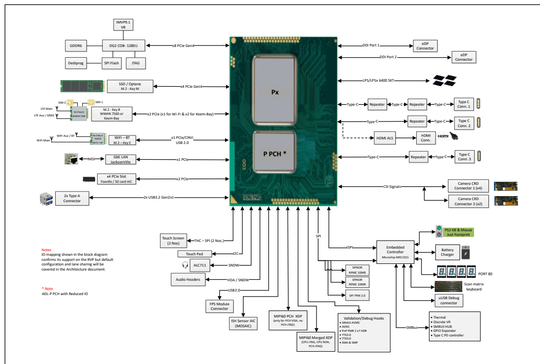
Figure 6. PX Processor Line Platform Diagram
