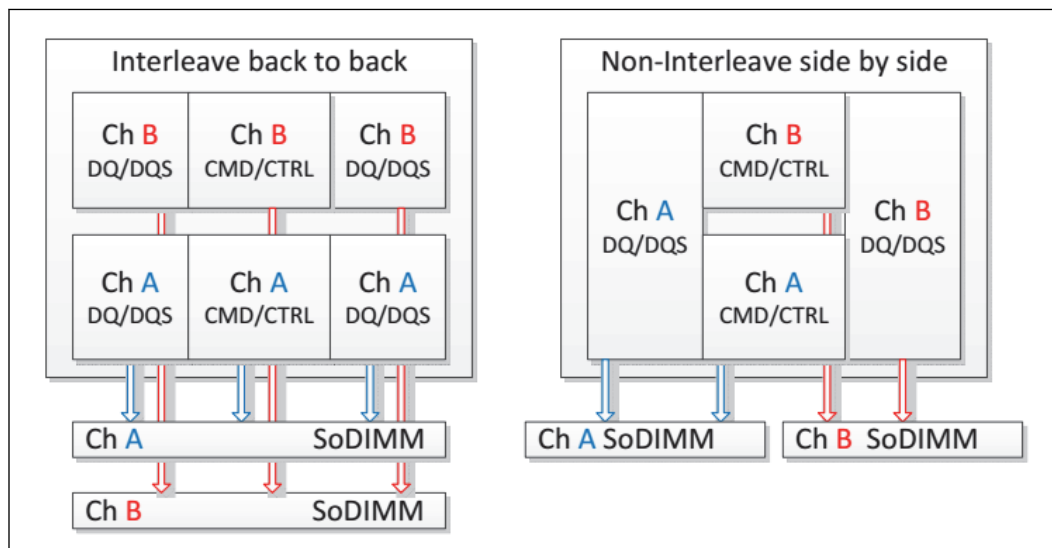
Figure 19. DDR4 Interleave (IL) and Non-Interleave (NIL) Modes Mapping
