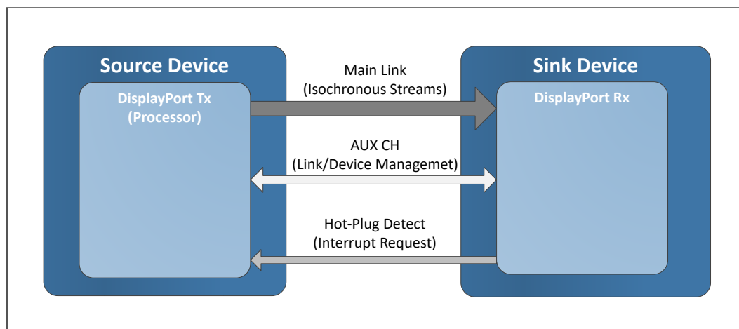
Figure 23. DisplayPort* Overview
