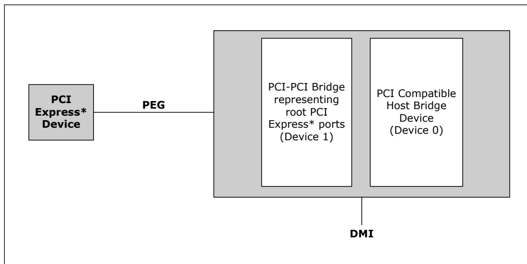
Figure 20. PCI Express® Related Register Structures in the Processor
