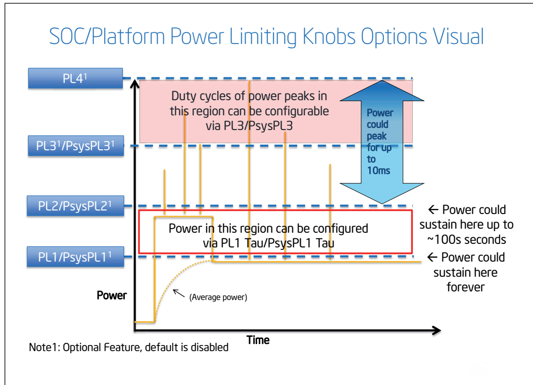
Figure 16. Package Power Control
