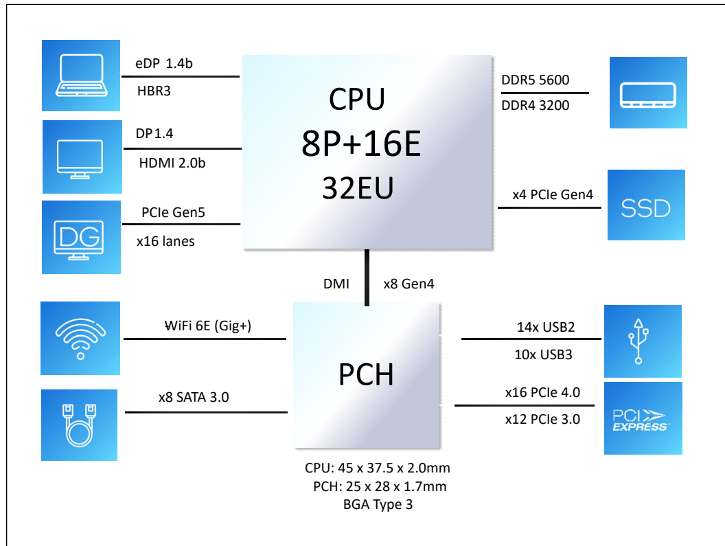
Figure 6. PX Processor Line Platform Diagram
